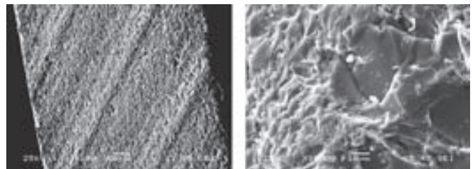
a) manually arrised edge, left: \times 100 ; right: \times 1000 very coarse abrasive size around 420 to 250 micron, (diamond wheel speed in rpm's 1600-2400) a) zámolt él, bal: \times 100 ; jobb: \times 1000
