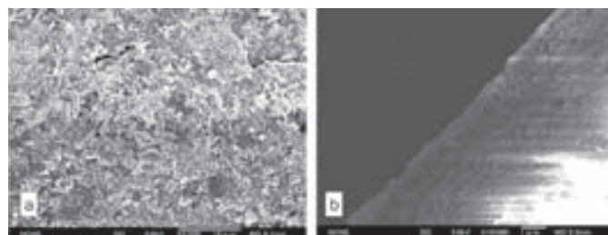
Fig. 1. SEM photographs of \text{AgVO}_3 coated silica gels produced at 400 °C (a) surface view and (b) cross sectional view
