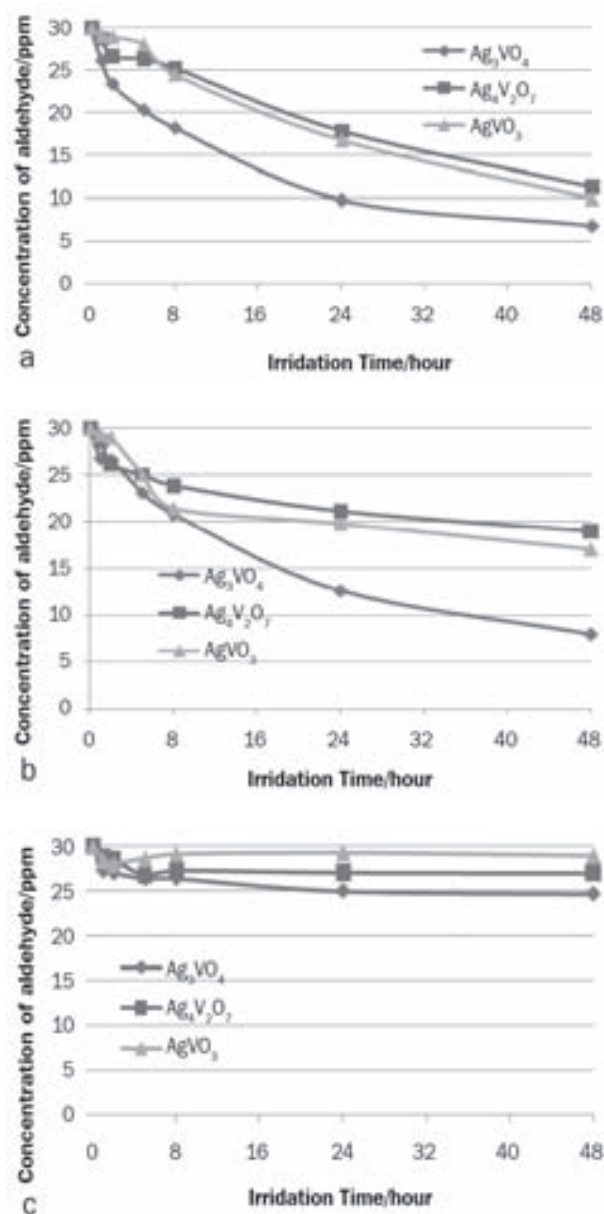
Fig. 3. Decomposition of acetaldehyde on Ag 2 O-V 2 O 5 powder mixture in (a) ultraviolet light, (b) fluorescent light and (c) in darkness
